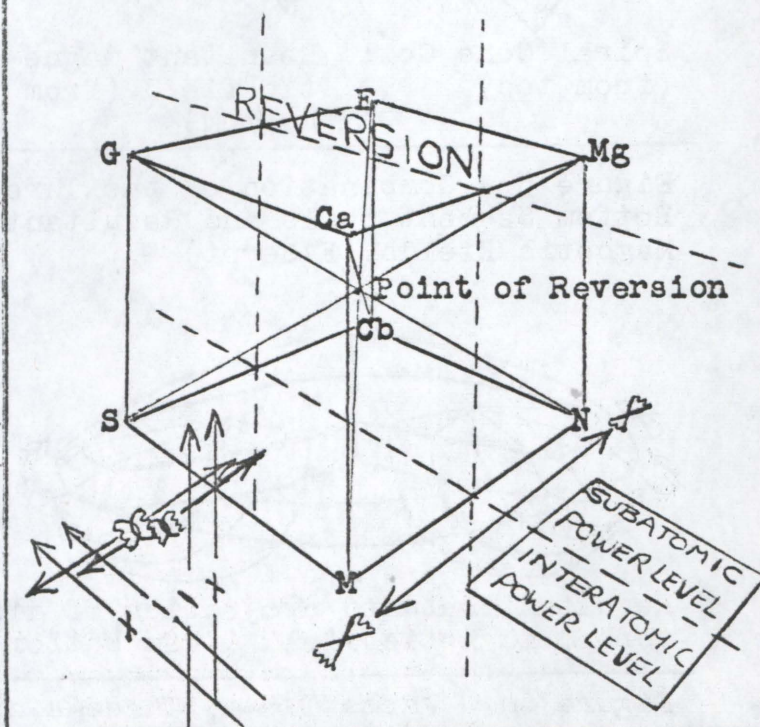
Figure 12 - Universal Forces and Their Relationships in a Reversional-Transitional Cosmos (Excerpt)
