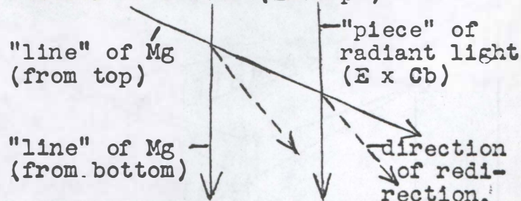
Figure 13C - Lengthly Spiral Form of Redirected Force Patterns. (Excerpt)
