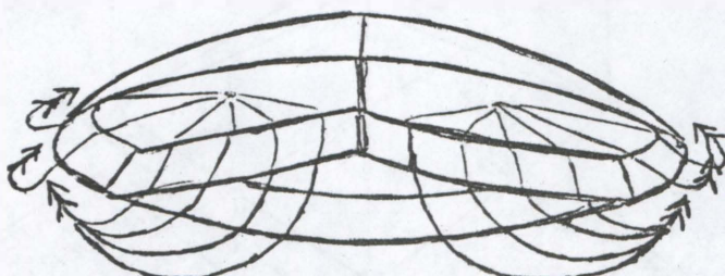
Resultant outward projection of disturbed magnetic field (from bottom).
