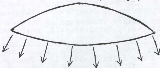
Figure 13A - Theoretic Course of Bottom Sphere-segment's Unaffected Radiant Magnetic Fields and Light. (Excerpt)
