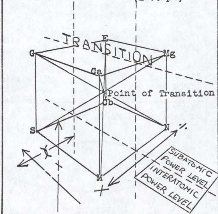
Figure 11 - Universal Forces and Their Relationships in a Transitional Mass-Energy Universe.
